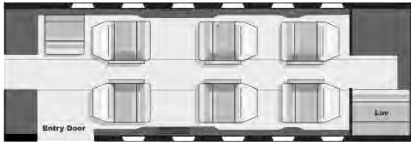
Scale = 1:50
